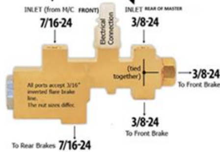
PROPORTIONING VALVE
