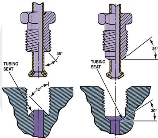
SAE Inverted Flare
